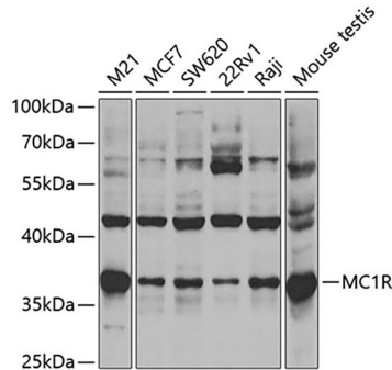
Fig. 1. Western blot analysis of extracts of various cell lines, using MC1R antibody at 1:400 dilution. Secondary antibody: HRP-labeled Goat Anti-Rabbit IgG(H+L) (A0208) at 1:1000 dilution. Lysates/proteins: 25µg per lane. Blocking buffer: QuickBlock™ Blocking Buffer (P0231). Detection: BeyoECL Star (P0018A). Exposure time: 1s.
